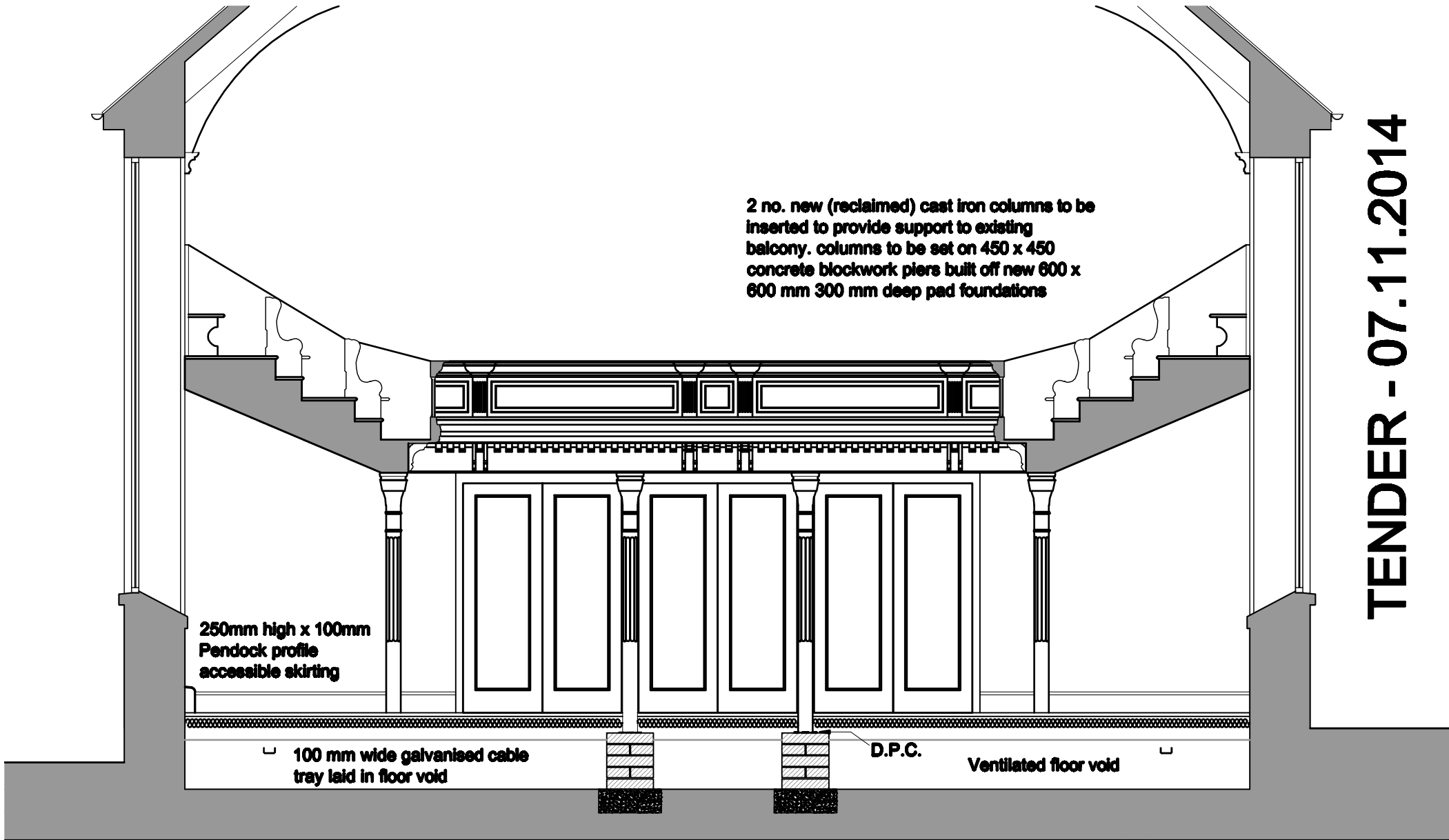
SECTIONAL ELEVATION SHOWING GLAZED DOORS TO LOBBY
